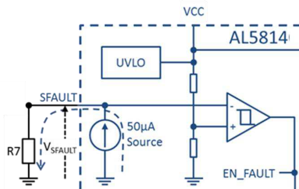
Figure 5. SFAULT Configuration
