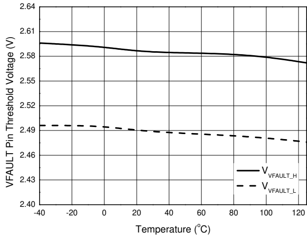
V_{FAULT} vs. Temperature
