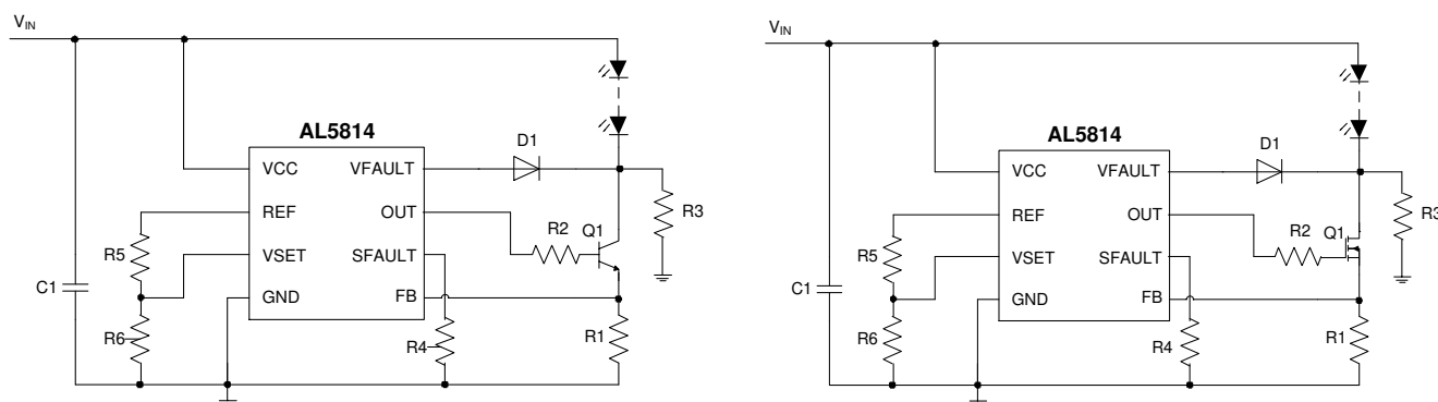
Figure 3. Typical Application
