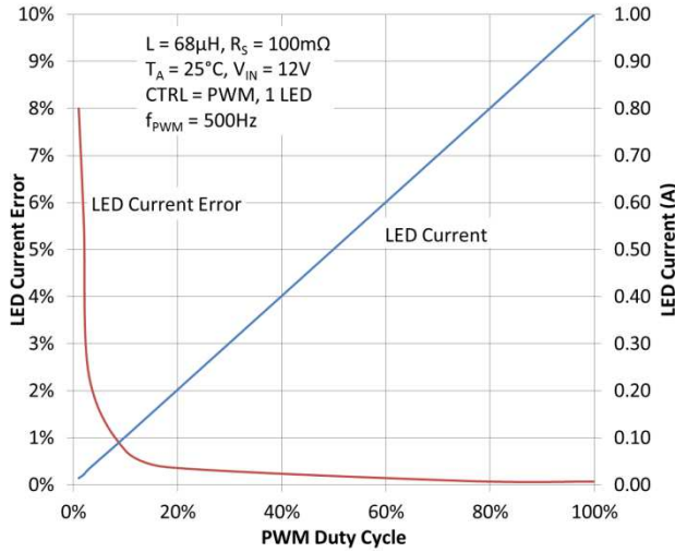
Figure 7. LED vs. PWM Duty Cycle
