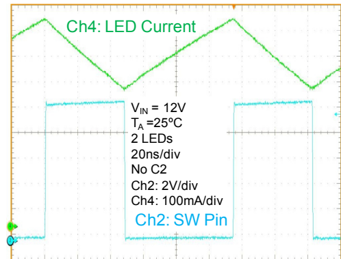
Figure 32 Typical Operating Waveform (C2 not fitted)
