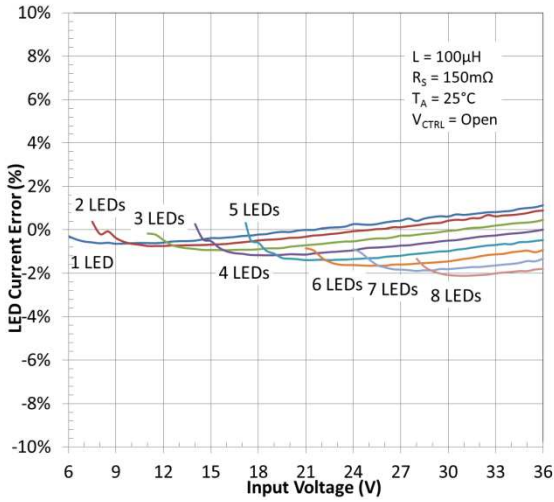
Figure 13. LED Current Deviation vs. Input Voltage
