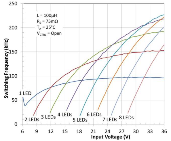
Figure 26. Switching Frequency vs. Input Voltage
