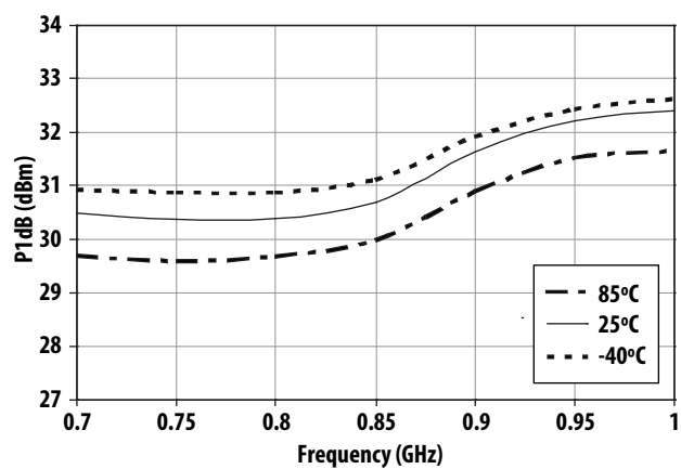
Figure 10. Over temperature P1dB vs Frequency
