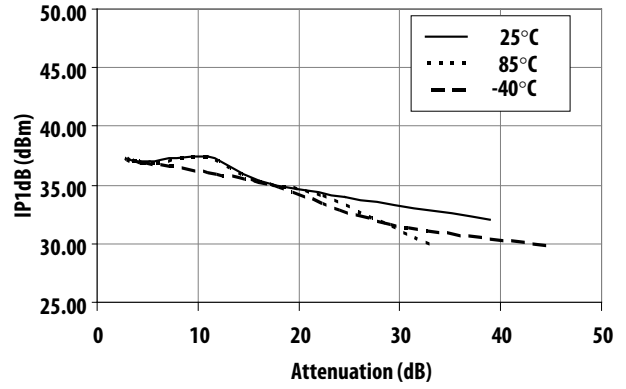
Figure 30. Input P1dB vs Attenuation vs Temperature at 1900MHZ
