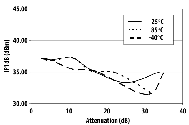
Figure 14. Input P1dB vs Attenuation vs Temperature at 1900MHZ
