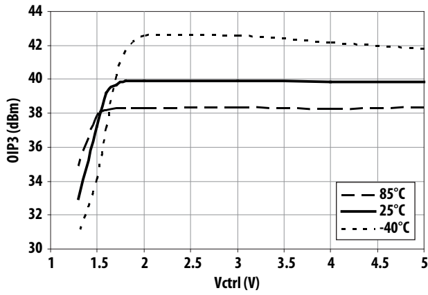
Figure 7. OIP3 vs Control Voltage and Temperature at 1900MHz
