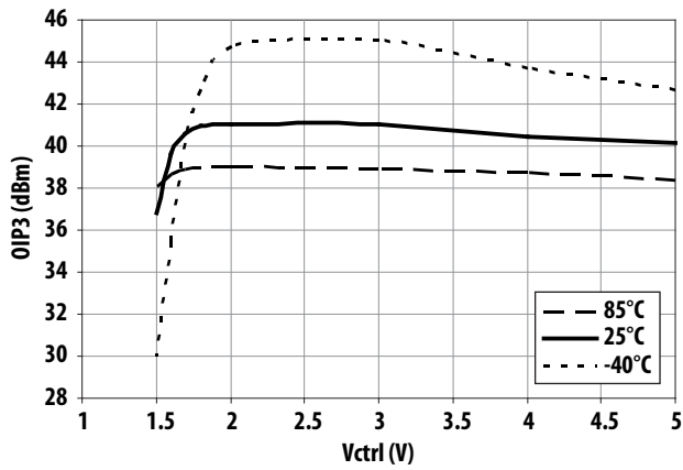
Figure 30. OIP3 vs Control Voltage and Temperature at 2500MHz
