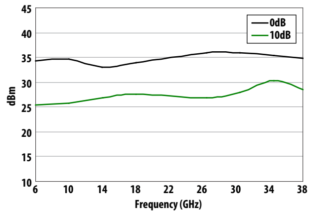
Figure 11. IIP3 vs Attenuation Input Power = 0dB
