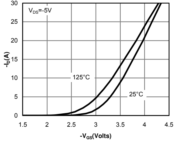
Figure 13: Transfer Characteristics
