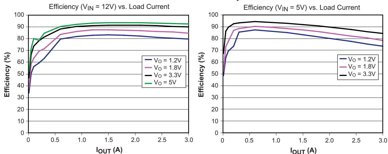
AOZ1031AI Efficiency
