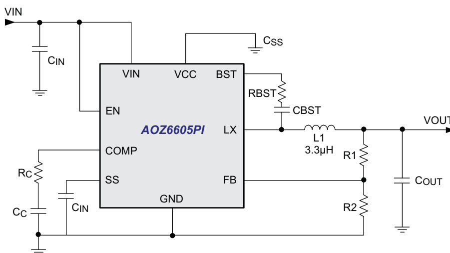
Figure 1. 5A Synchronous Buck Regulator, F_s = 650\text{kHz}
