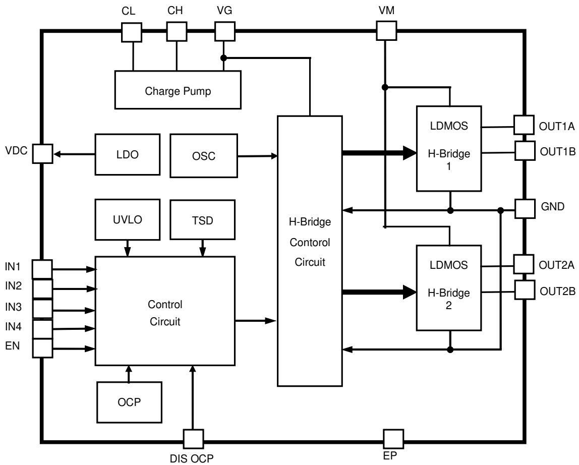
Figure 1. Block Diagram
