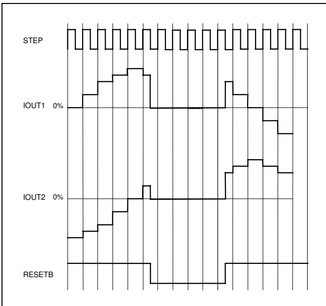
Figure 6. RESETB signal Timing Chart (W1-2 phase)
