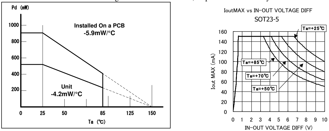
Figure 6. SOT23-5
