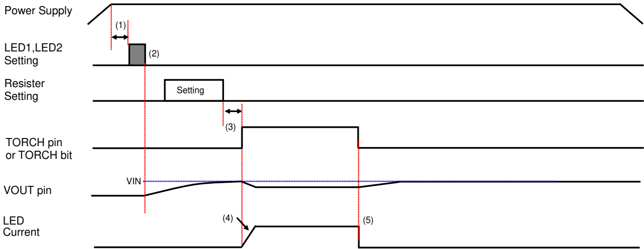
Figure 6. Torching Sequence
