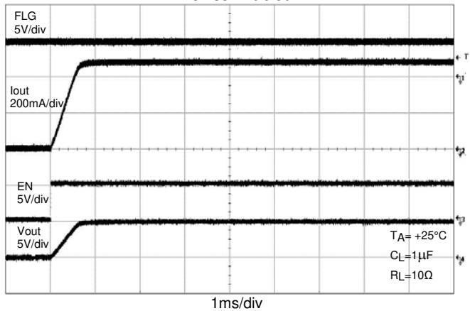
UVLO Increasing
