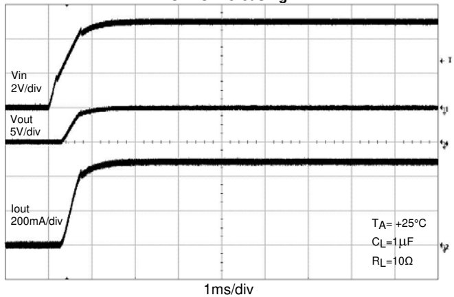
UVLO Increasing
