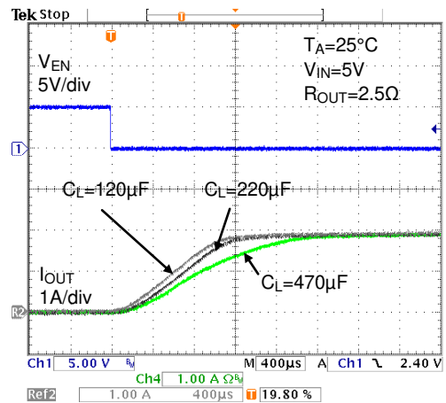
Inrush Current
