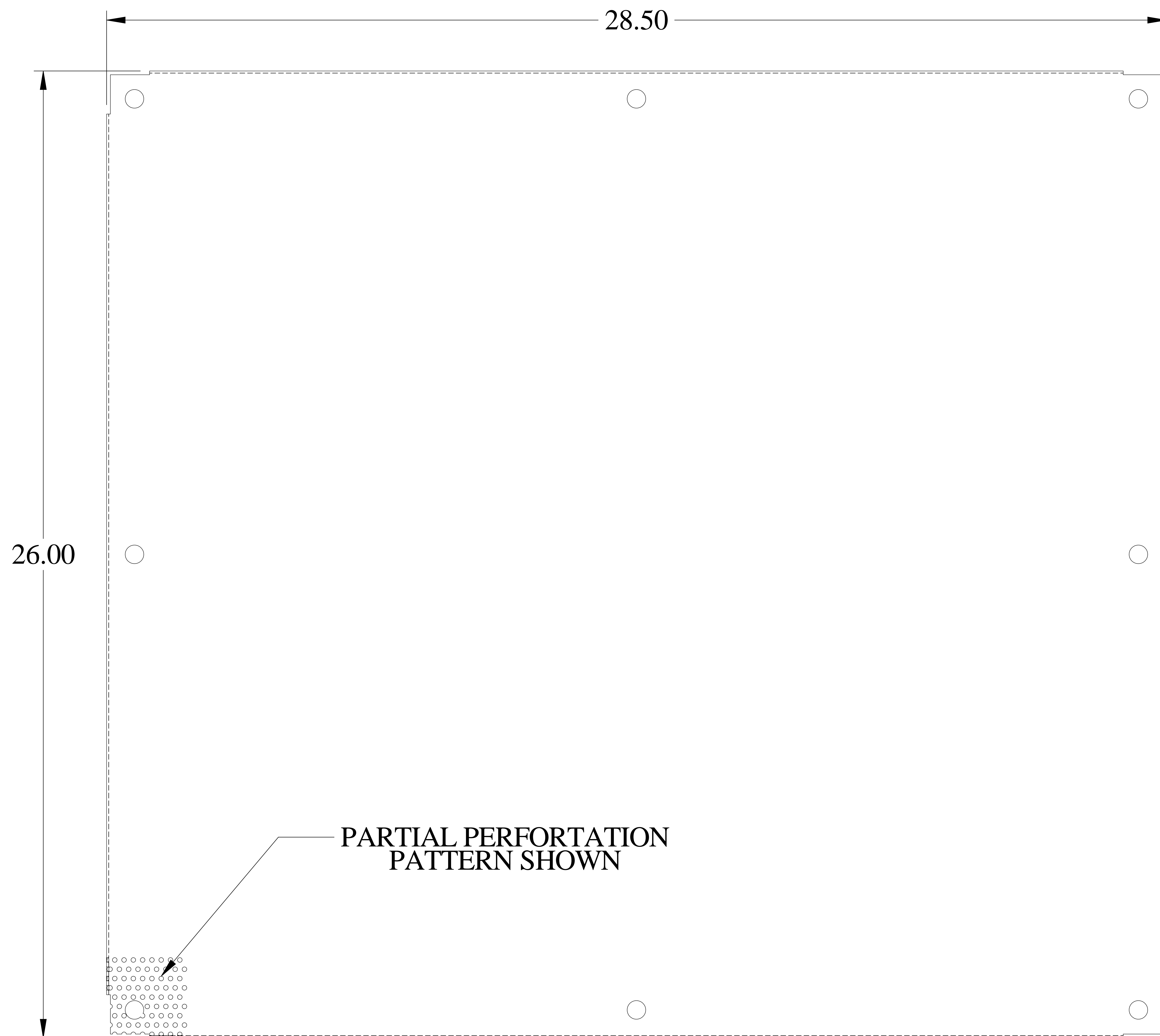
FRONT VIEW
