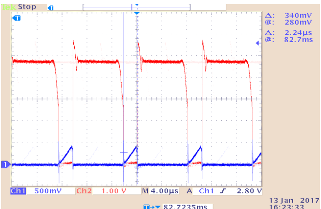
Fig:11 Vds & Vcs at 264V AC at FL 100V/Div
