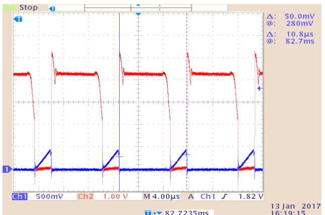
Fig:10 Vds & Vcs at 230V AC at FL 100V/Div
