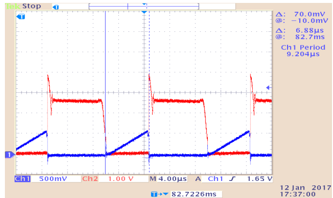
Fig:9 Vds & Vcs at FL at 115V AC 100V/Div
