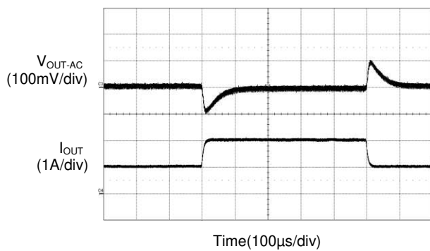
Load Transient Response ( I_{OUT}=1A to 2A )
