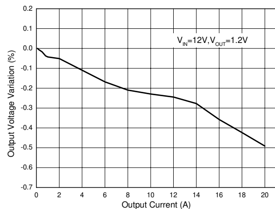
Figure 5. Load Regulation
