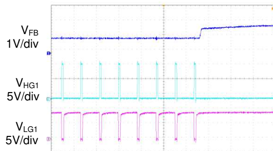
Time 4μs/div
