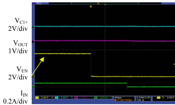
Time (400μs/div)
