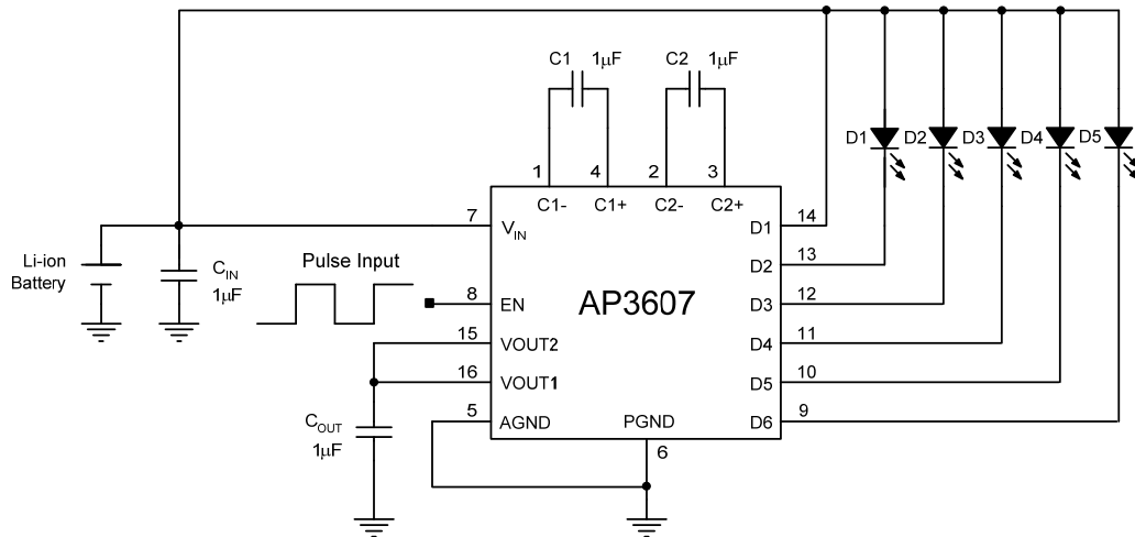
5 WLEDs
