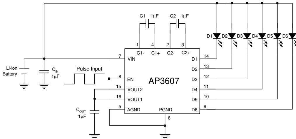
6 WLEDs
