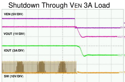
Time-50μs/div
