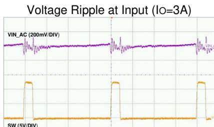
Time-400ns/div
