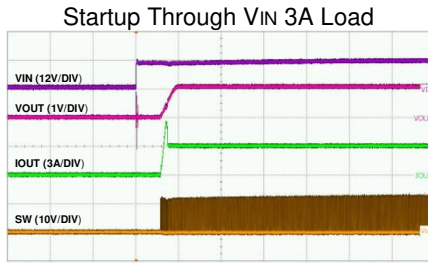
Time-1ms/div
