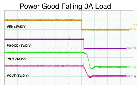
Time-50μs/div
