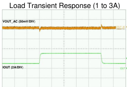
Time-100μs/div
