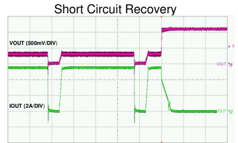
Time-1ms/div
