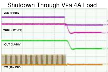
Time-50μs/div
