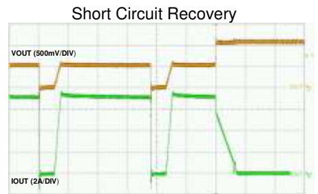
Time-1ms/div
