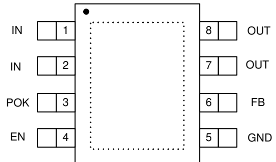
SOP-8L-EP
