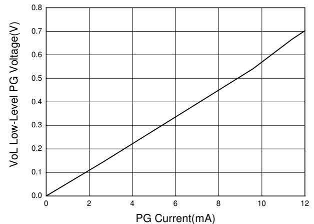
Figure 14 Low-Level PG Voltage vs Current
