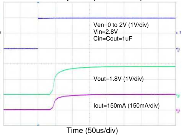
Start-Up Time (150mA Load)
