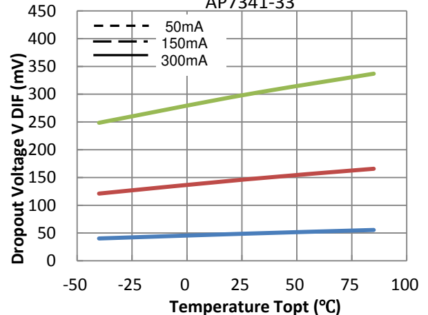
Dropout Voltage vs. Temperature AP7341-33
