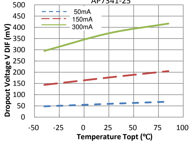
Dropout Voltage vs. Temperature AP7341-25
