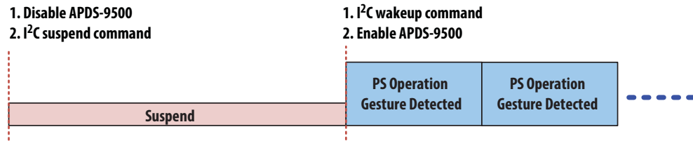
Figure 21. Suspend State (SUS) Diagram.
