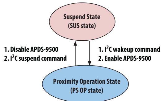
Figure 22. State Machine of Gesture Detection.
