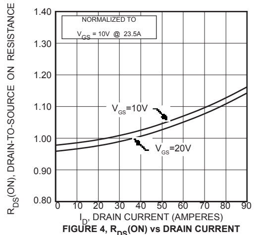
FIGURE 4, R_{DS(\text{ON})} vs DRAIN CURRENT
