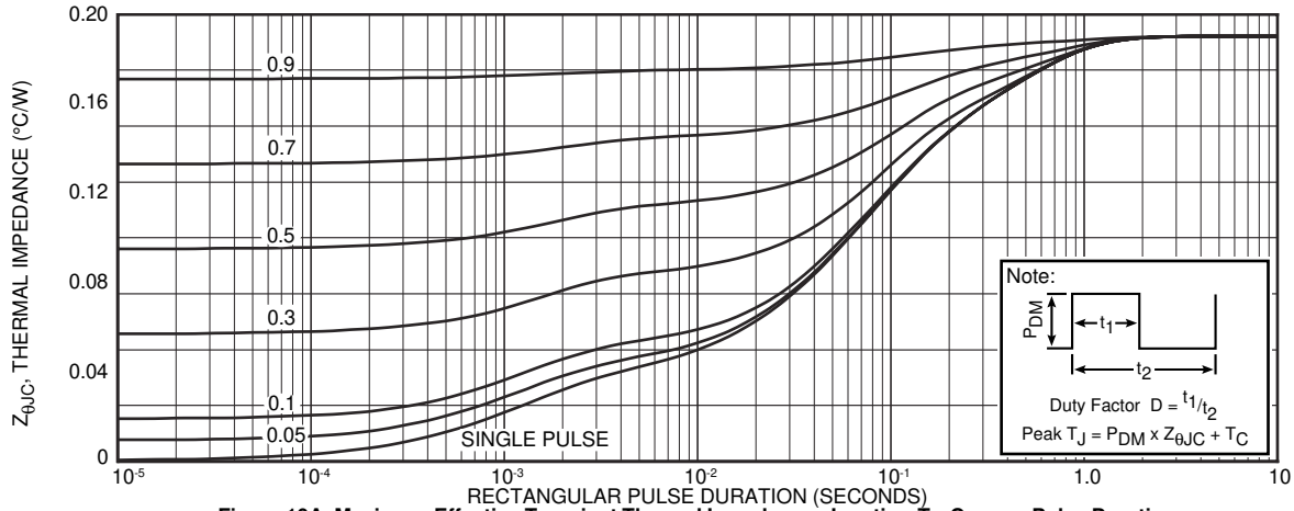
Figure 19A, Maximum Effective Transient Thermal Impedance, Junction-To-Case vs Pulse Duration
