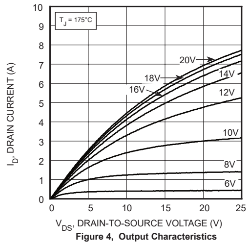
Figure 4, Output Characteristics
