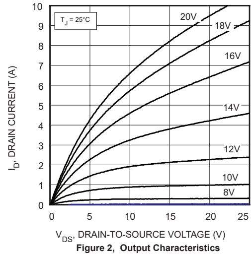
Figure 2, Output Characteristics
