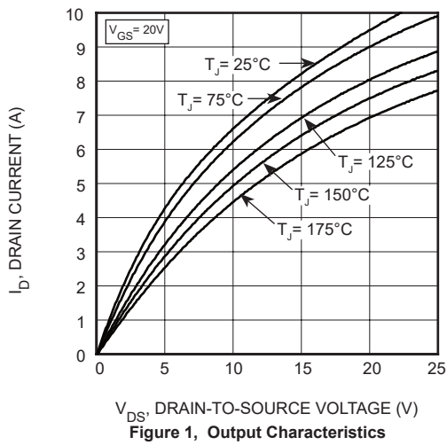
Figure 1, Output Characteristics
