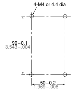
Mounting dimensions (Bottom view)
