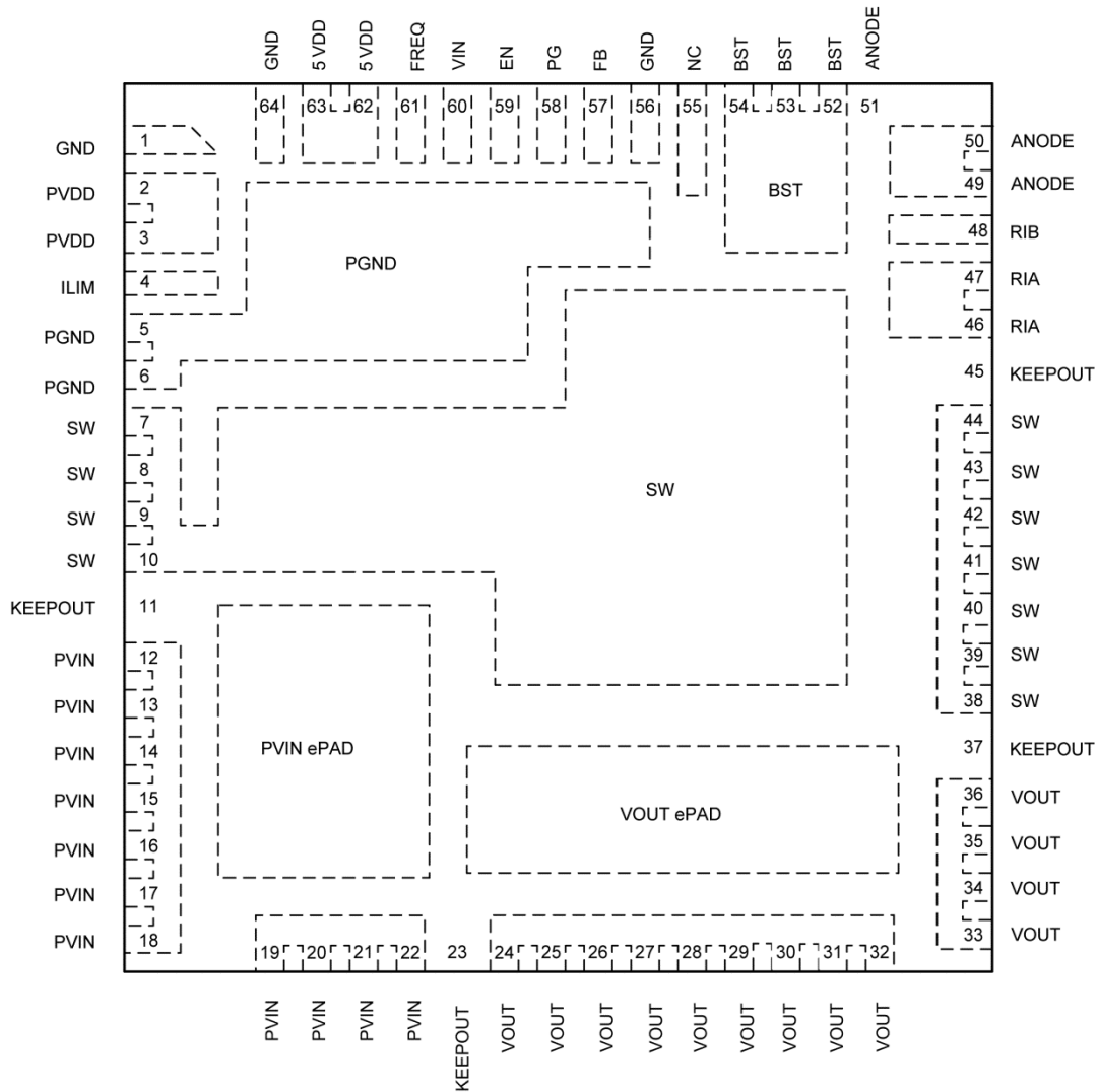
64-Pin 12mm × 12mm × 4mm QFN (Top View)
