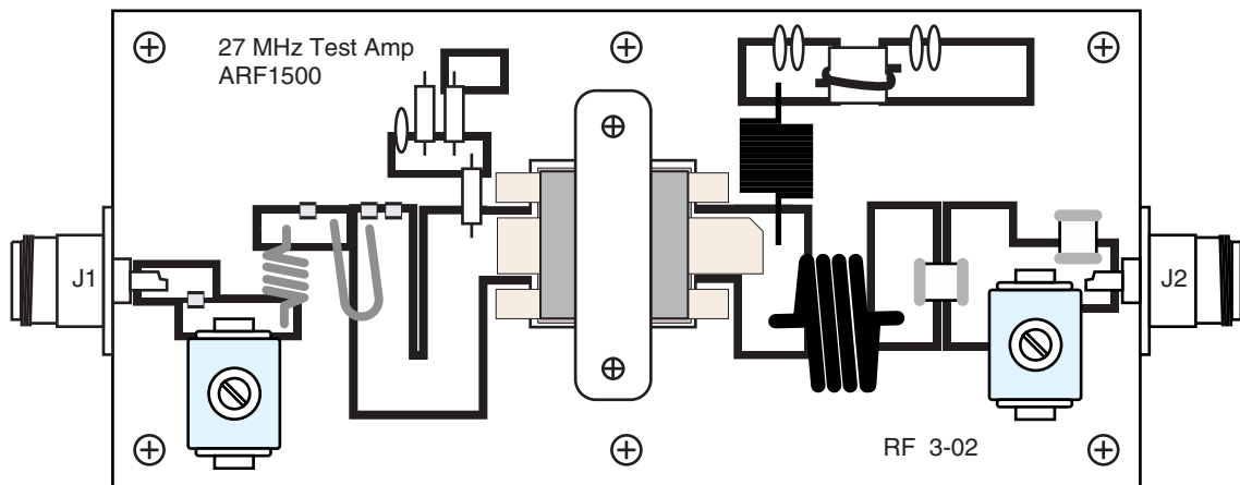
Parts placement
