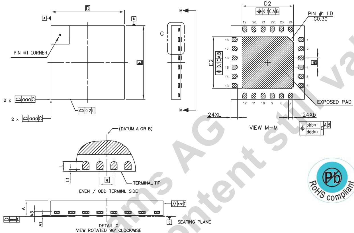
Figure 28. TQFN(4x4)-24 Package
