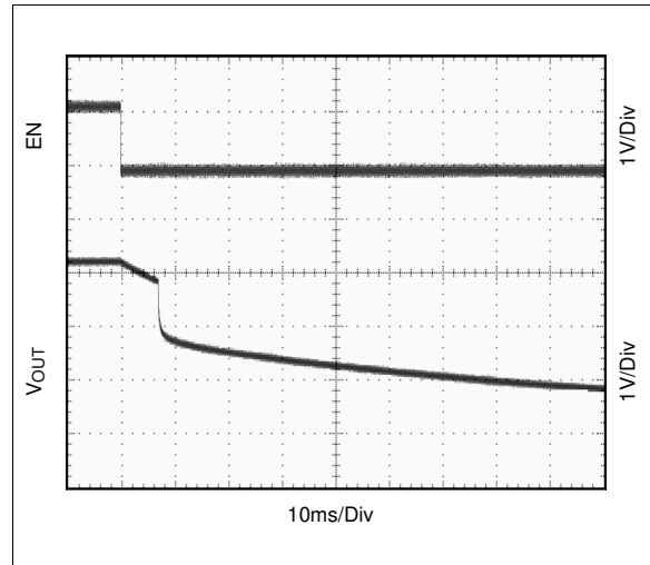
Figure 22. Shutdown Voltage, I_{OUT} = 1\text{mA}
