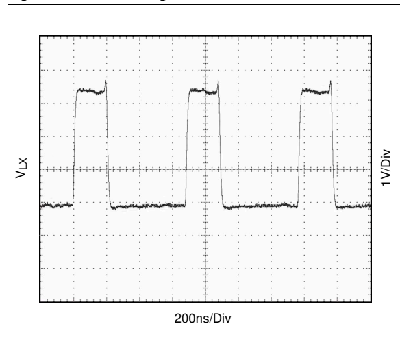
Figure 24. Coil Voltage, I_{OUT} = 100\text{mA}
