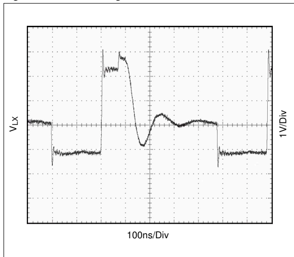
Figure 23. Coil Voltage, I_{OUT} = 1\text{mA}
