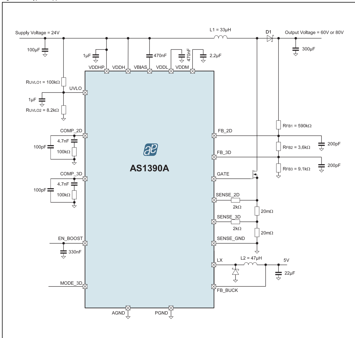
Figure 22. Typical Application
