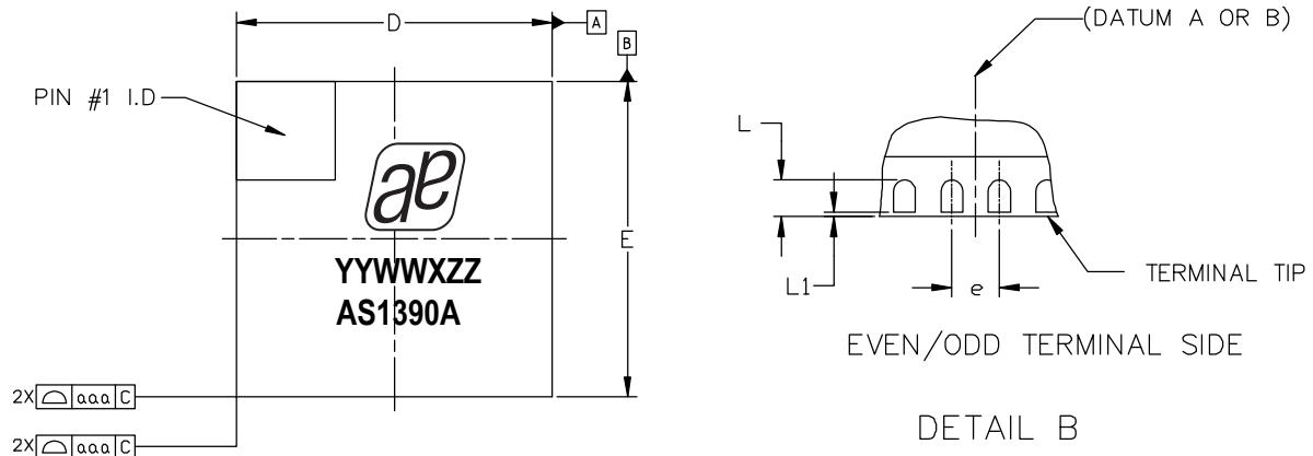
Figure 23. 20-pin QFN (4x4mm) Package
