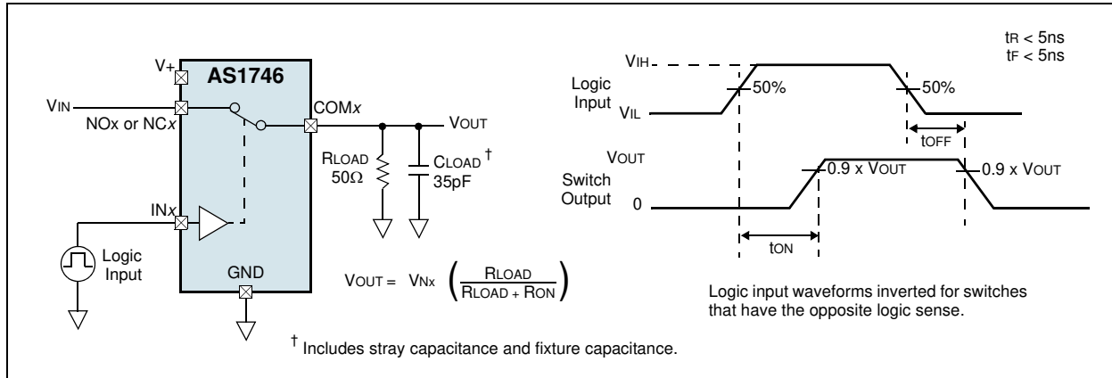
Figure 17. Switching Time
