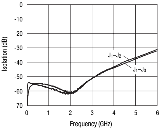
Isolation, -40 °C V_{DD} = 5\text{ V}, V_{CTL} = 0/5\text{ V}
