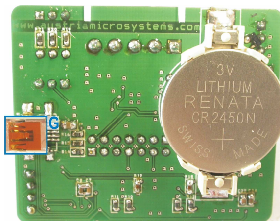
Figure 2: Board Description Bottom – Connectors
