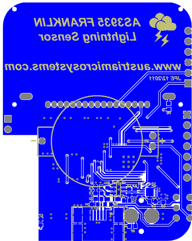
Figure 8: Bottom Layer
