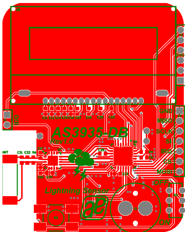
Figure 7: Top Layer
