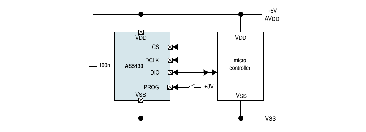
Figure 7. Serial Data Transmission in Continuous Readout Mode
