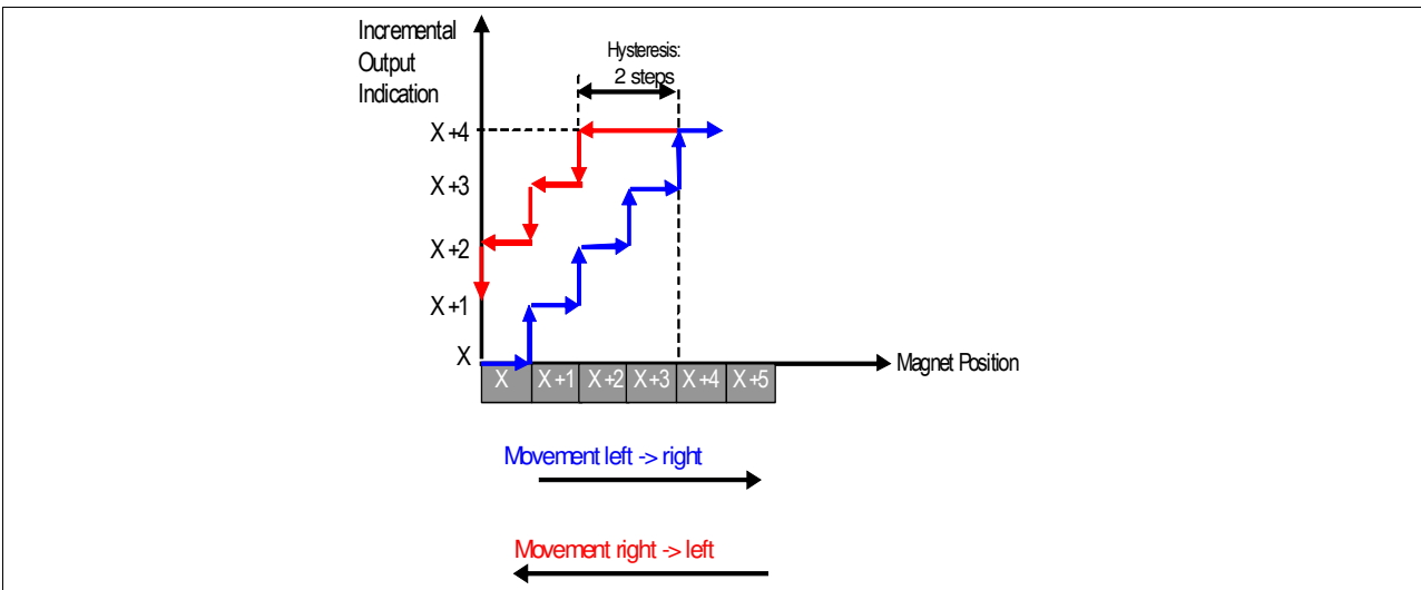
Figure 7. Hysteresis Illustration
