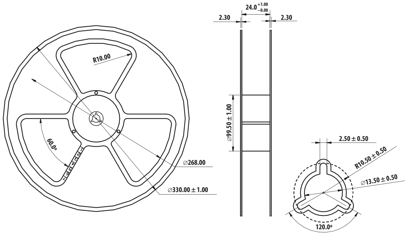
Figure 18. Reel dimensions.
