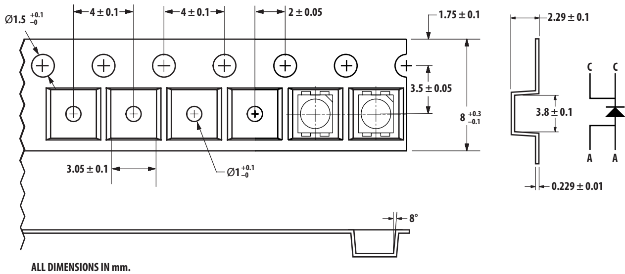
Figure 16. Tape Dimensions
