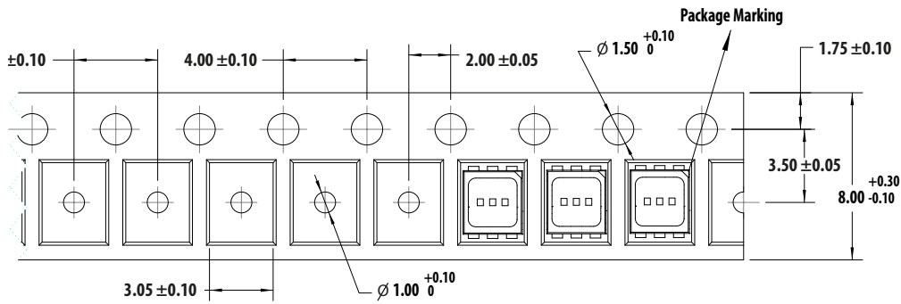
Figure 16 Reeling Orientation
