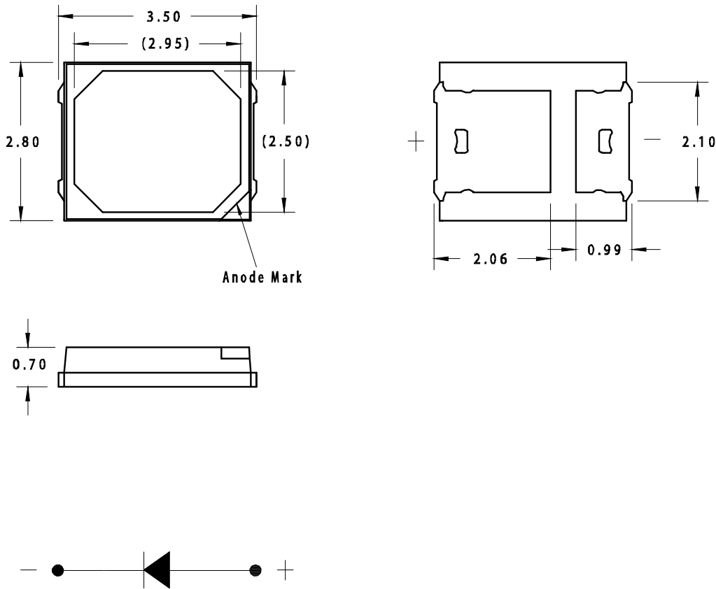
Figure 1 Package Dimensions
