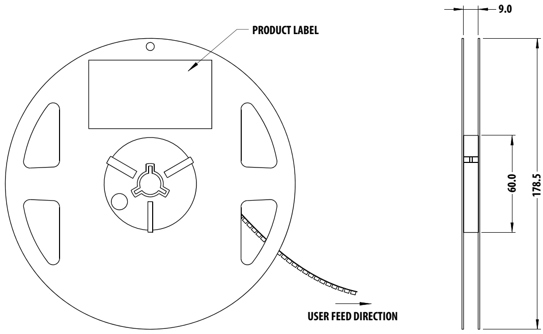
Figure 15 Reel Dimension
