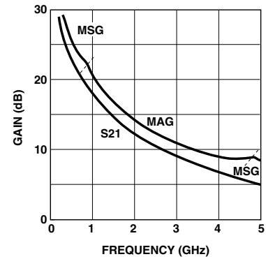
Figure 25. AT-32011 Gains vs. Frequency at V_{CE} = 5 V , I_C = 20 mA .
