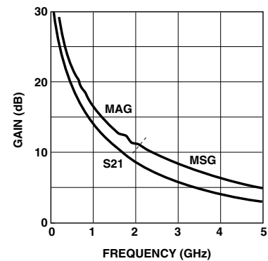
Figure 26. AT-32033 Gains vs. Frequency at V_{CE} = 5 V , I_C = 20 mA .
