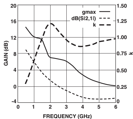
Figure 9. Gain vs. Frequency at 1 V, 1 mA.
