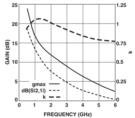
Figure 15. Gain vs. Frequency at 5 V, 10 mA.
