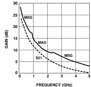
Figure 11. AT-41533 Gains vs. Frequency at V_{CE} = 2.7 V , I_C = 5 mA .
